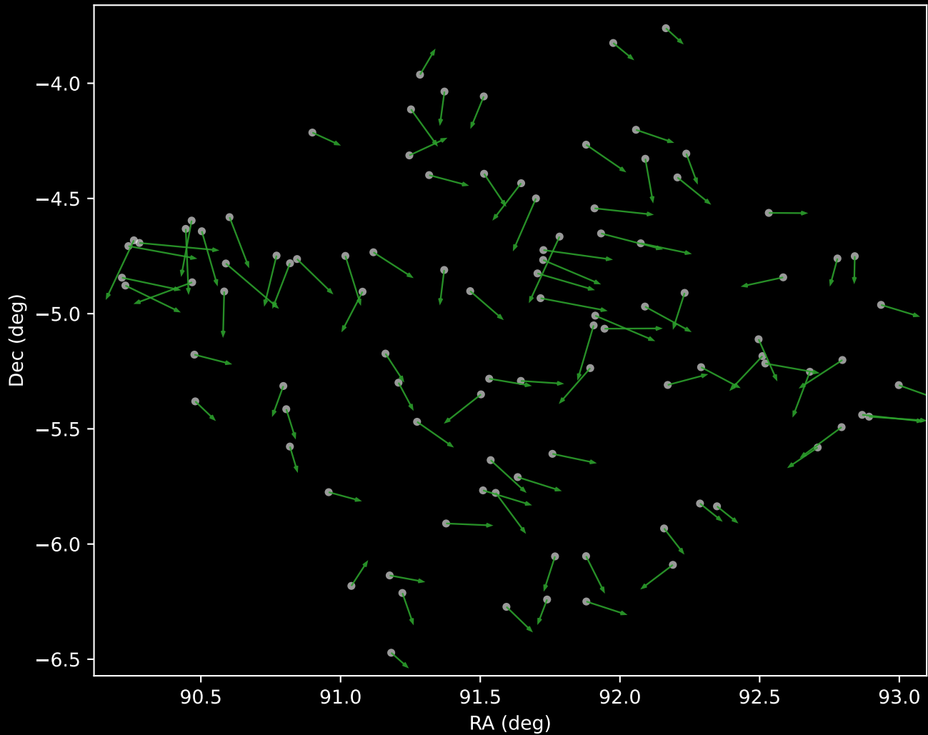
APOGEE DR17 Cluster 4 Proper Motion Vectors (n=99)
