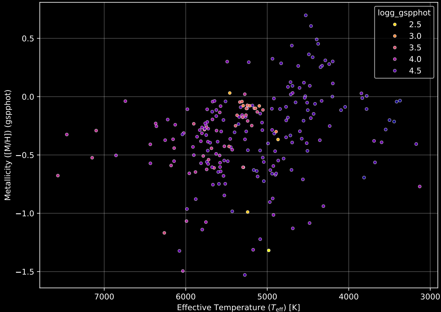
APOGEE DR17 Field: [K2_C12_077-60_btx] Stellar Population Parameters (n= 229)
