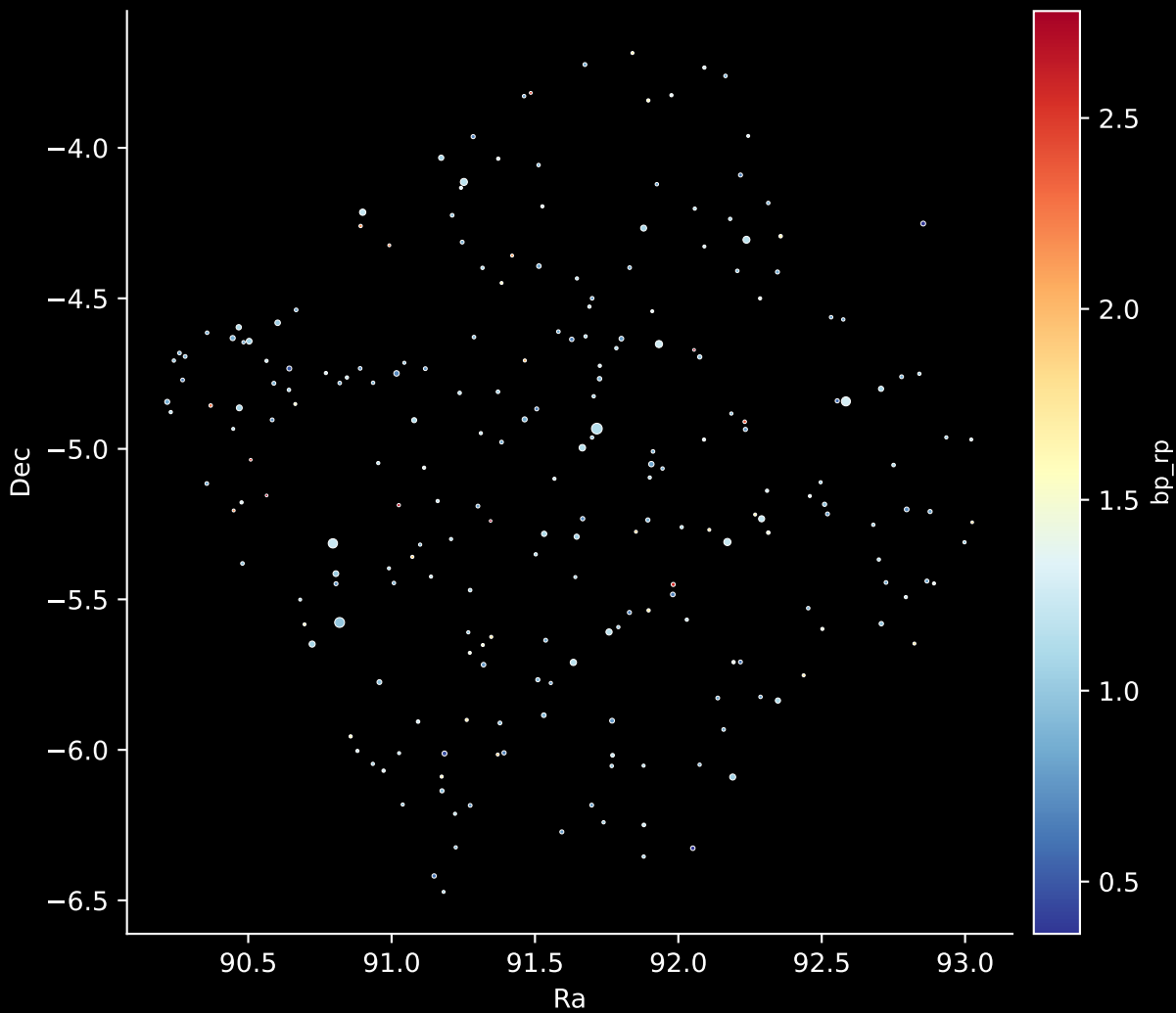
APOGEE DR17 Field: [K2_C12_077-60_btx] Stars: 229
