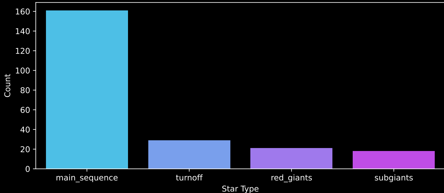
APOGEE DR17 Field: [K2_C12_077-60_btx] Count plot of Star Type
