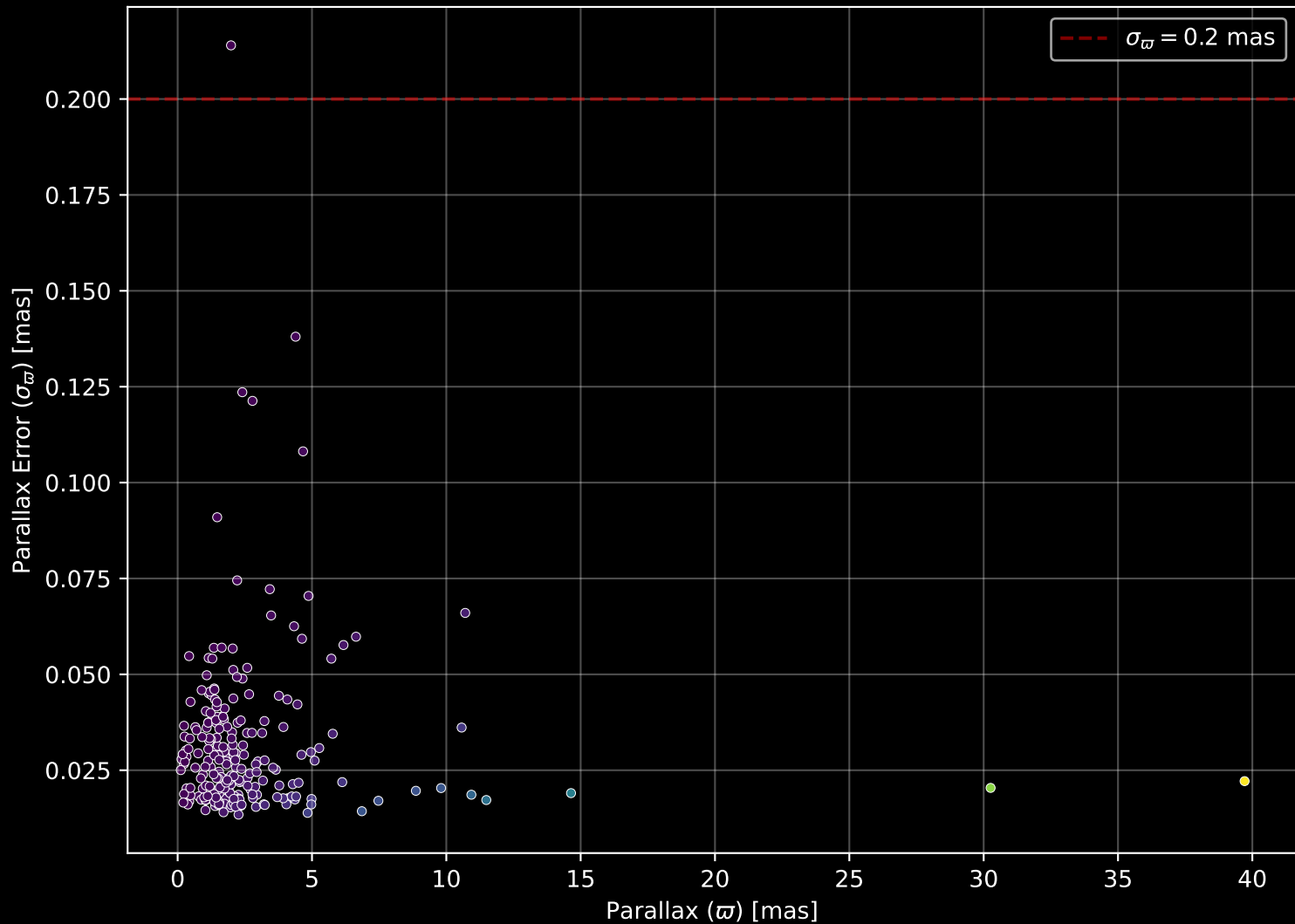
APOGEE DR17 Field: [K2_C12_077-60_btx] Parallax Quality (n= 229)
