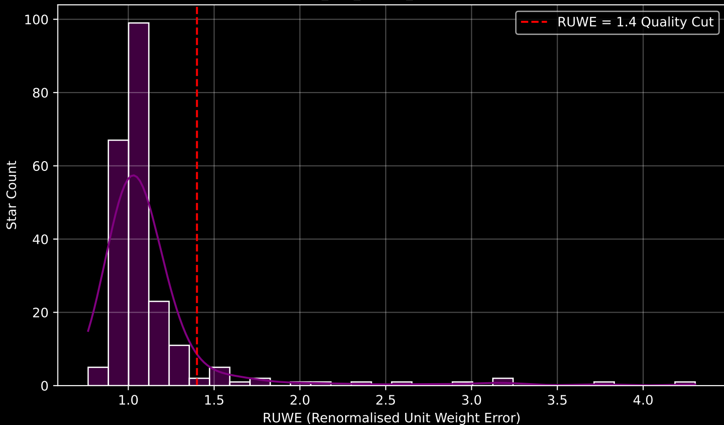
GAPOGEE DR17 Field [K2_C12_077-60_btx] RUWE Distribution (n= 224)
