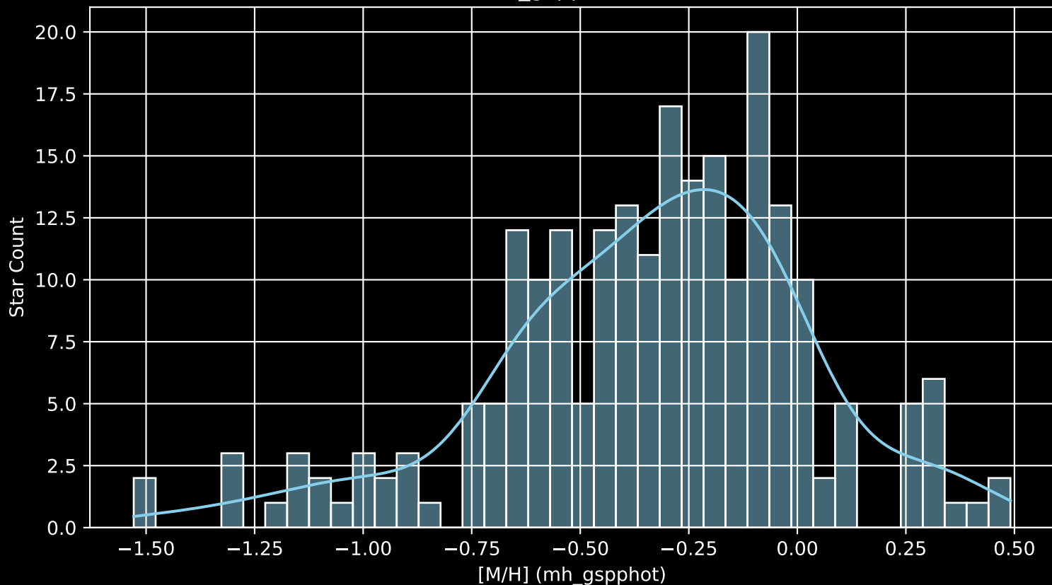
APOGEE DR17 Field: [K2_C12_077-60_btx [M/H] (mh_gspphot) (n= 227)
