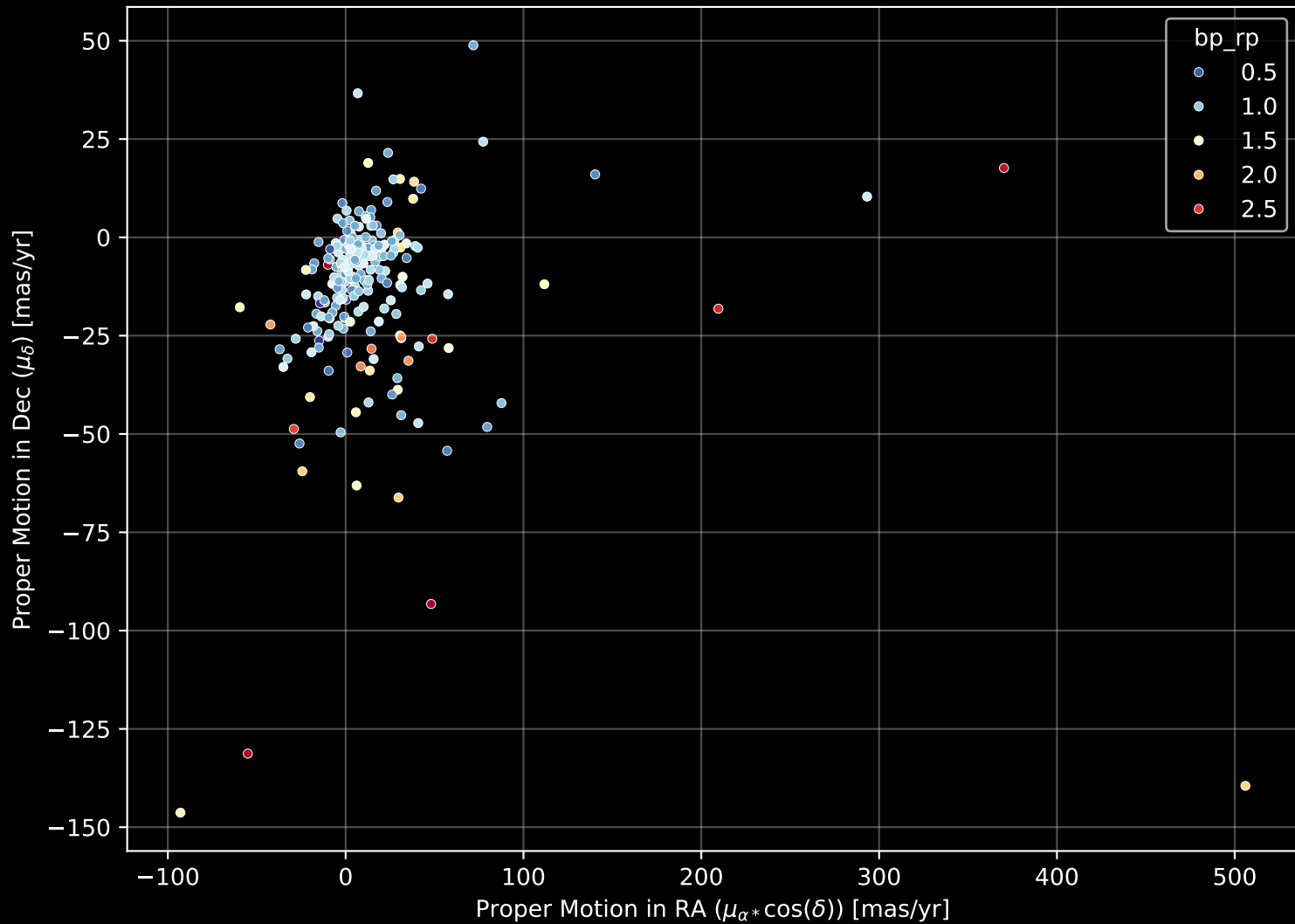
APOGEE DR17 Field: [K2_C12_077-60_btx] Proper Motion Diagram (n= 229)
